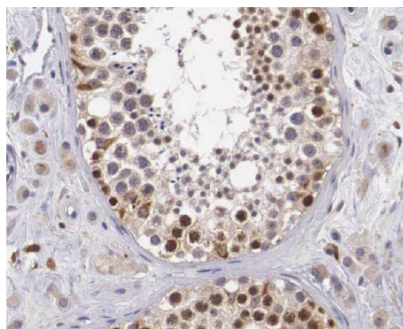
Immunohistochemistry of paraffin-embedded human testis using FNab09474(WBP2 antibody) at dilution of 1:50
